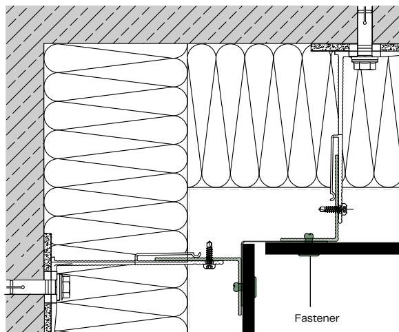
Internal corner A106
