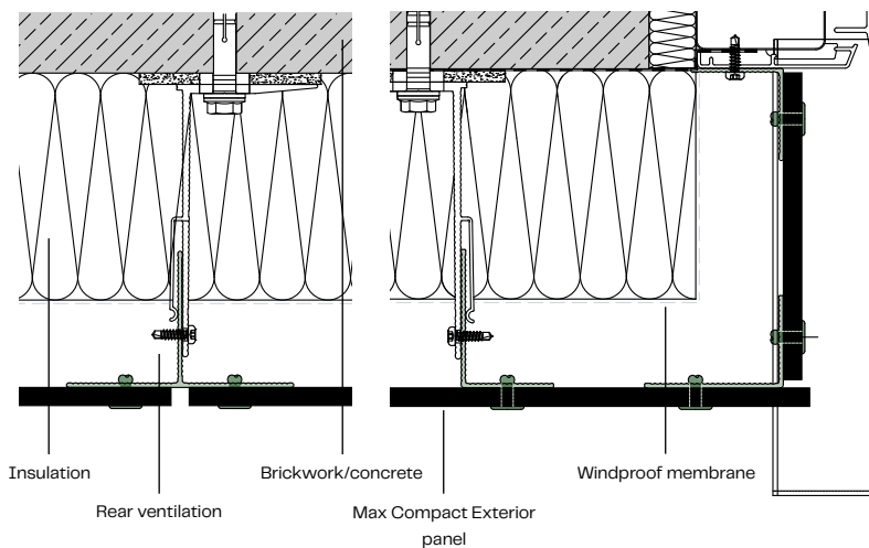
Vertical joint A107
